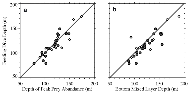
Fig. 5. Eubalaena glacialis and Calanus finmarchicus . Average depth of feeding dive versus (a) average depth of peak C. finmarchicus C5 abundance and (b) average depth of the bottom mixed layer. (●) Tagged whales that had 2 or more feeding dives with accompanying CTD/OPC casts. (◊) Tagged whales that had only 1 feeding dive with an accompanying CTD/OPC cast
