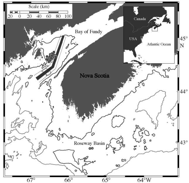
Fig. 2. Map of study area. (●) Tagging locations in the lower Bay of Fundy and Roseway Basin. Shipping lanes through the lower Bay of Fundy at the time of this study and the 91 m (50 fathom) and 200 m isobaths are also shown
